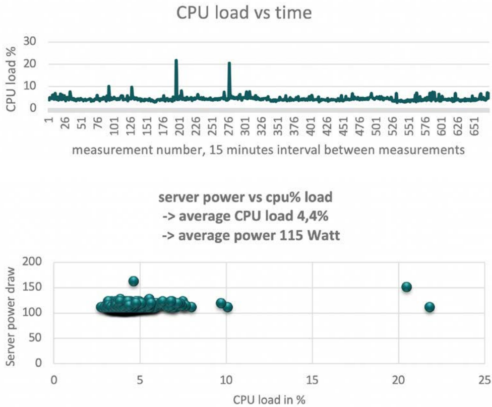
Figure 12: underloaded server configured as “static high performance”.
