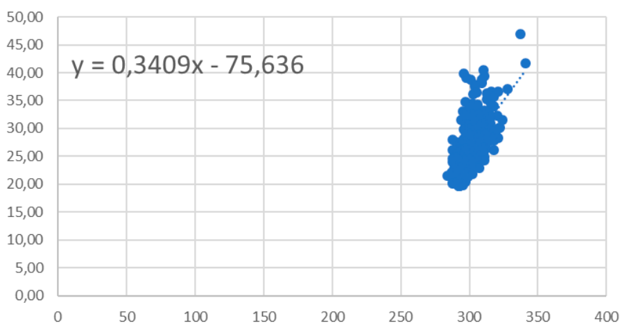
Figure 8: server 1, power save setting. In this graph, the vertical axis shows the CPU load of the server and the horizontal axis shows the power that was measured. Each point corresponds to a measurement interval where both CPU loading and power data were collected. (for example, 25% load, 300 Watt).
