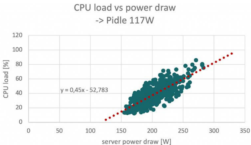
figure 14: cpu load vs power for server 669 in balanced mode, Pidle from extrapolation 117 Watt
