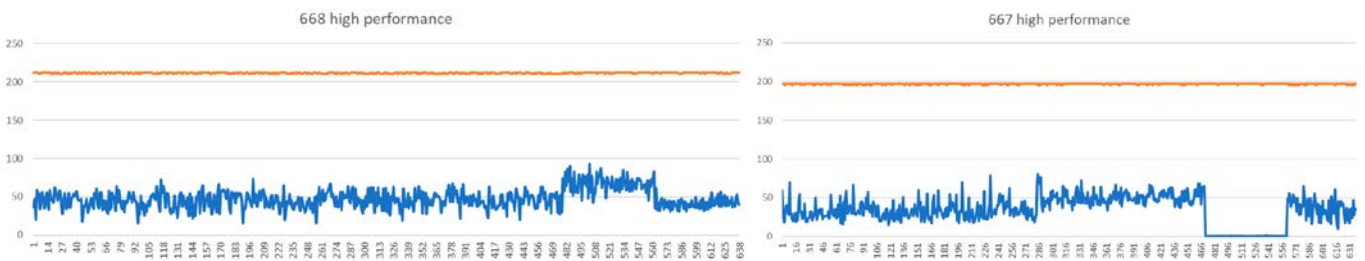
Figure 4: two servers in static high performance mode. In these graphs, the vertical axis has a double meaning. The blue line shows the CPU load as a percentage from 0% (idle) to 100% (fully loaded), the orange line shows the electrical power draw P in Watt. The horizontal axis just shows the number of the measurement interval.
