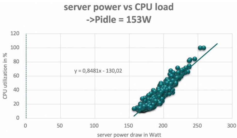
Figure 13: CPU load vs power draw. Server in OS-Control mode running VMware with a balanced profile
