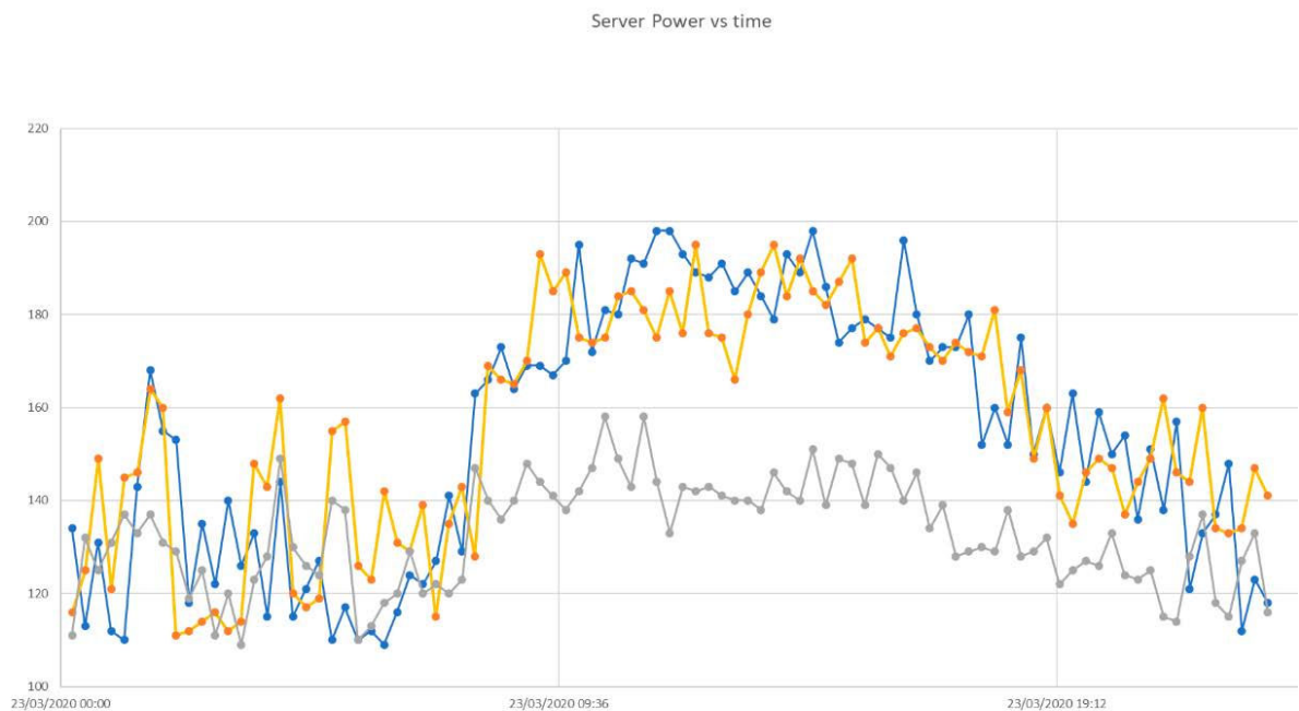
Figure 17: Measurements under high performance and balanced
