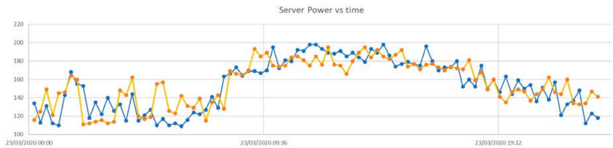
Figure 16: Power draw of server, Blue line hardware controlled, orange line OS controlled
