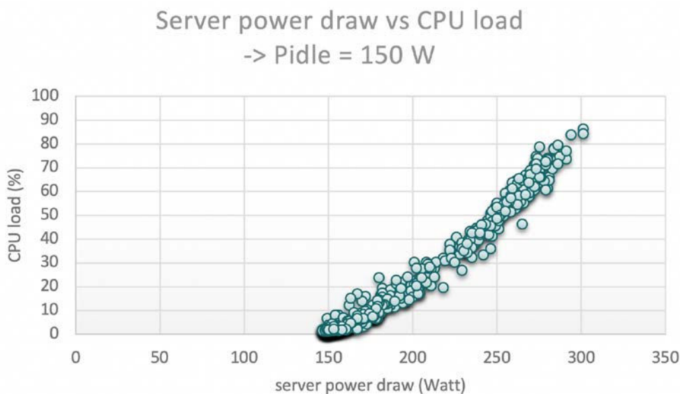
Figure 11: Power vs CPU load
