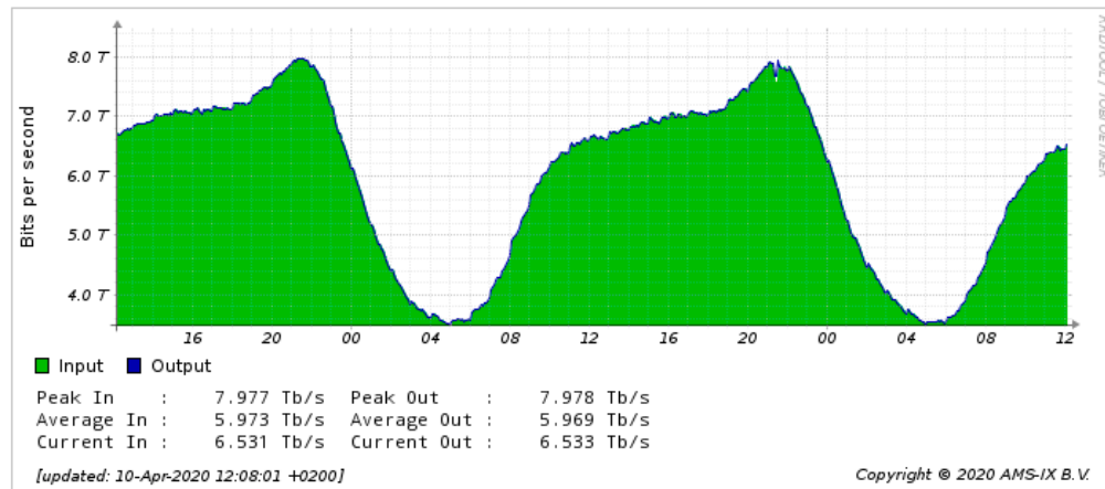
Figure 3: AMS-IX daily traffic
