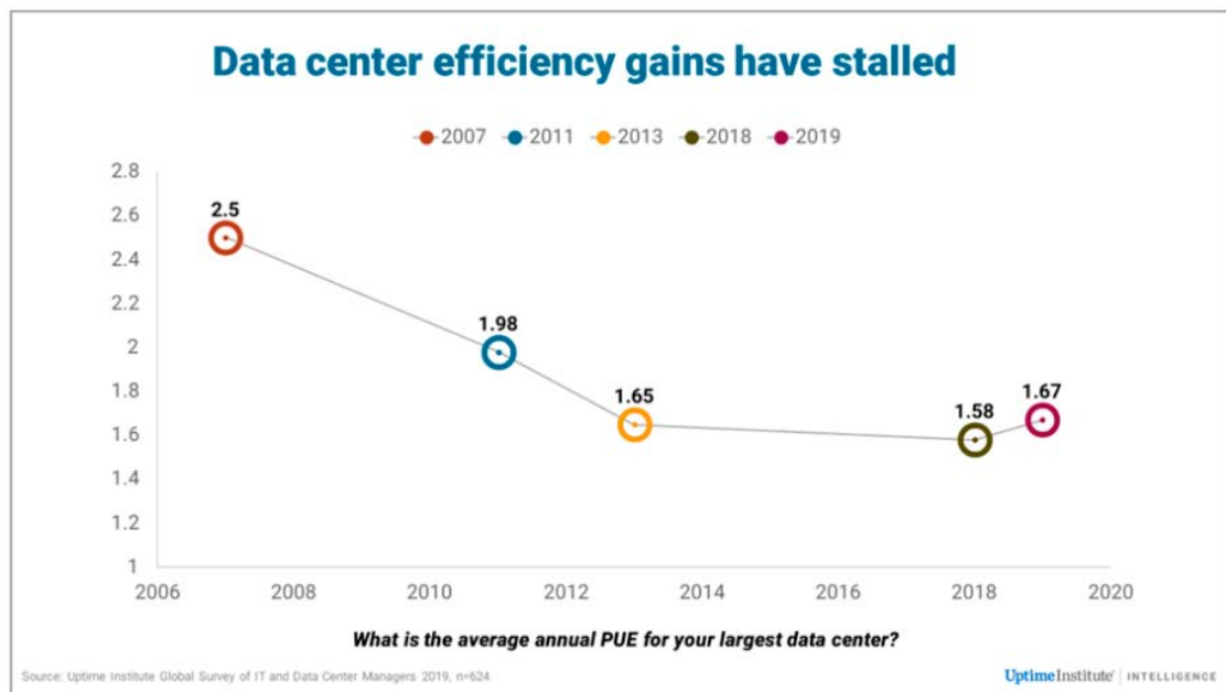
Figure 1: worldwide average PUE over the years
